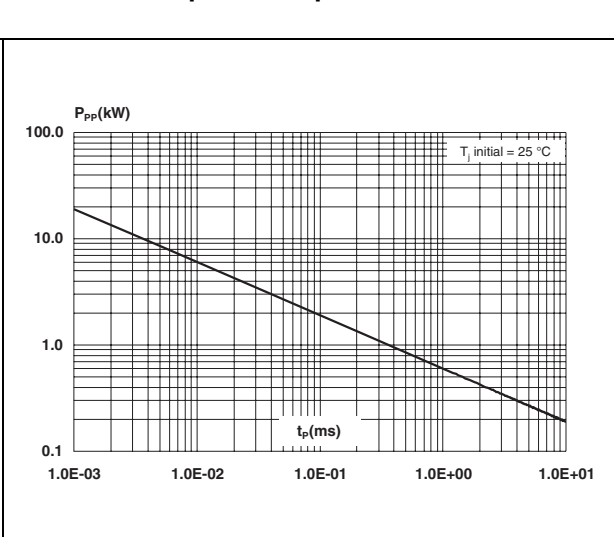
Figure 4. Peak pulse power versus exponential pulse duration
