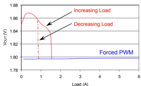
Figure 24. Power-Saving Mode Regulation (Using Figure 10 Circuit)
