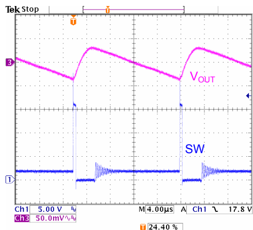
Figure 16. SW and V_{OUT} Ripple, 0.3A Load
