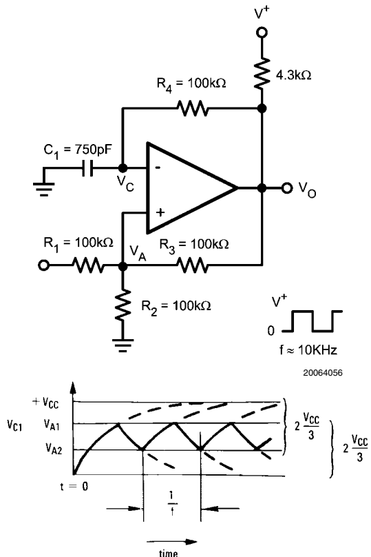
FIGURE 10. Squarewave Oscillator
