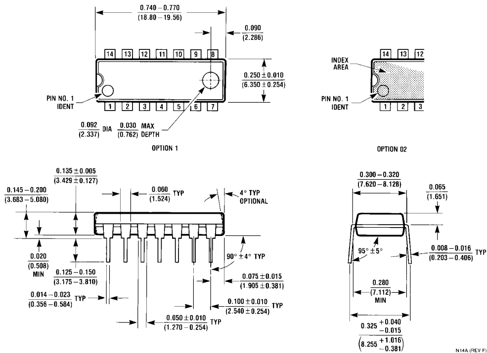
14-Pin Molded Dual-In-Line Package (N) Order Number LMC6084AIN or LMC6084IN NS Package Number N14A
