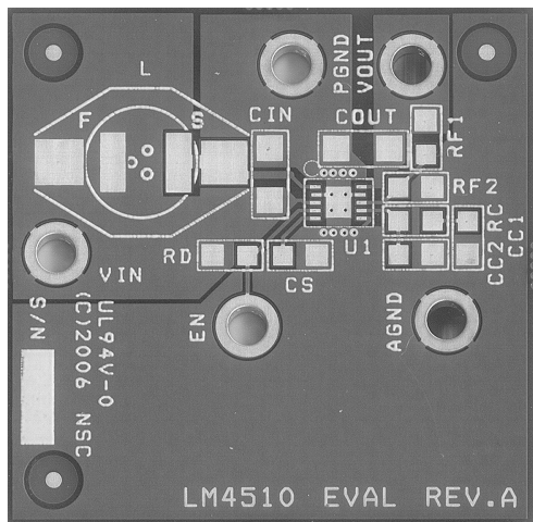
FIGURE 7. Evaluation Board Layout
