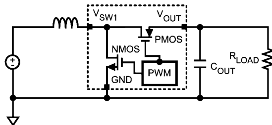
FIGURE 3. Schematic of Synchronous Boost Converter
