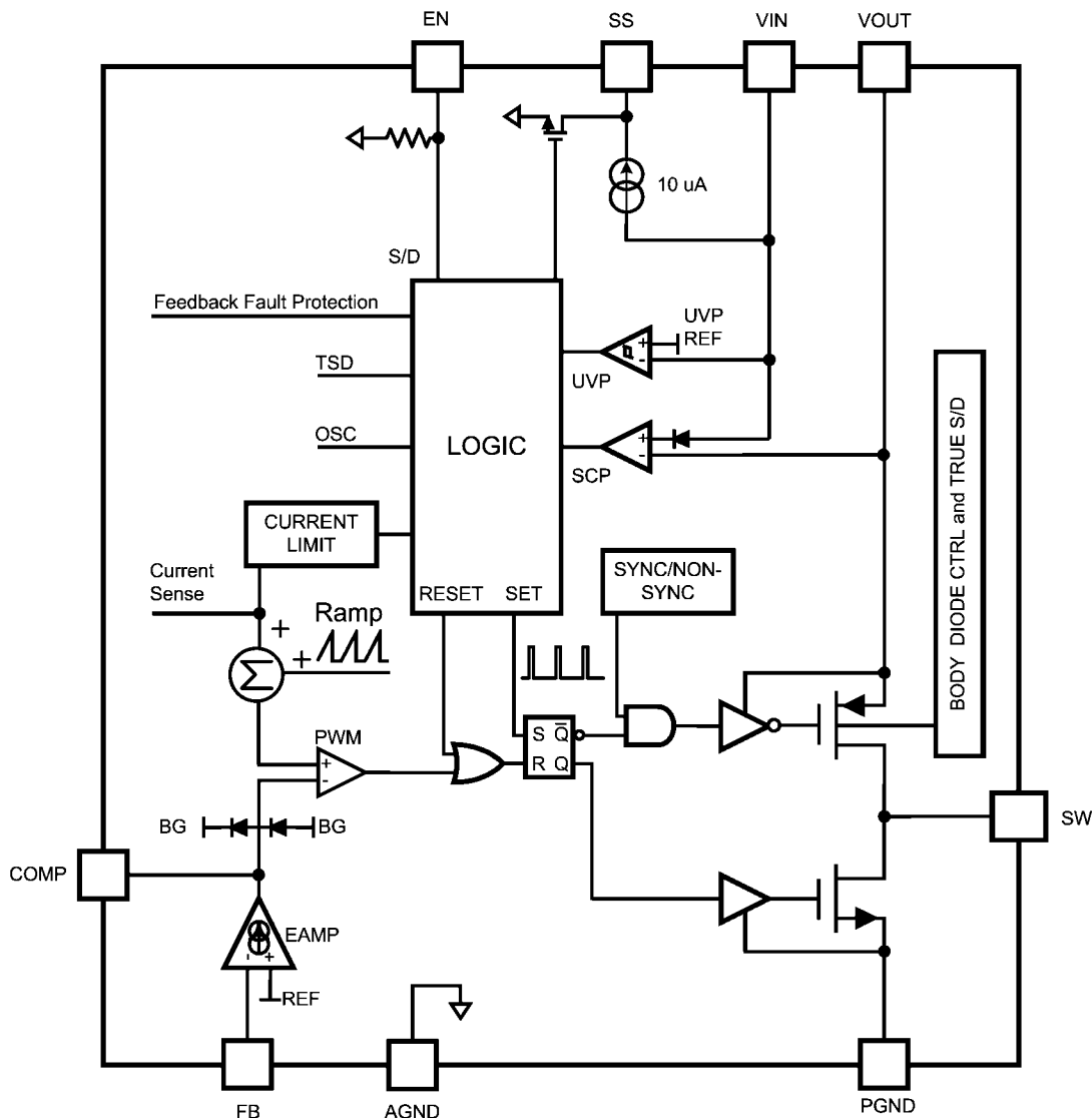
FIGURE 2. LM4510 Block Diagram
