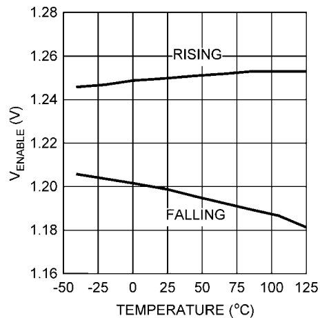
EN Threshold and Hysteresis vs. Temperature
