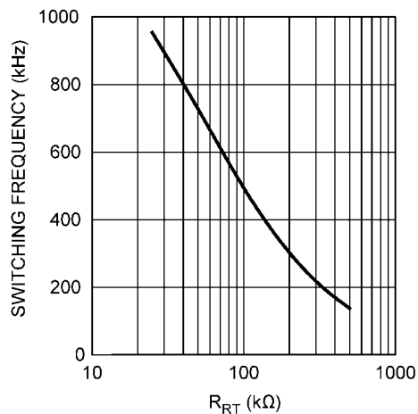
Oscillator Frequency vs. R_{RT}
