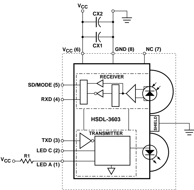
Figure 1. HSDL-3603 functional block diagram.
