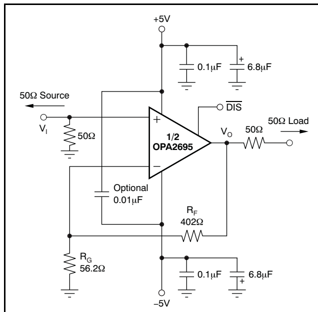
Figure 68. DC-Coupled, G = +8\text{V/V} , Bipolar Supply Specifications and Test Circuit
