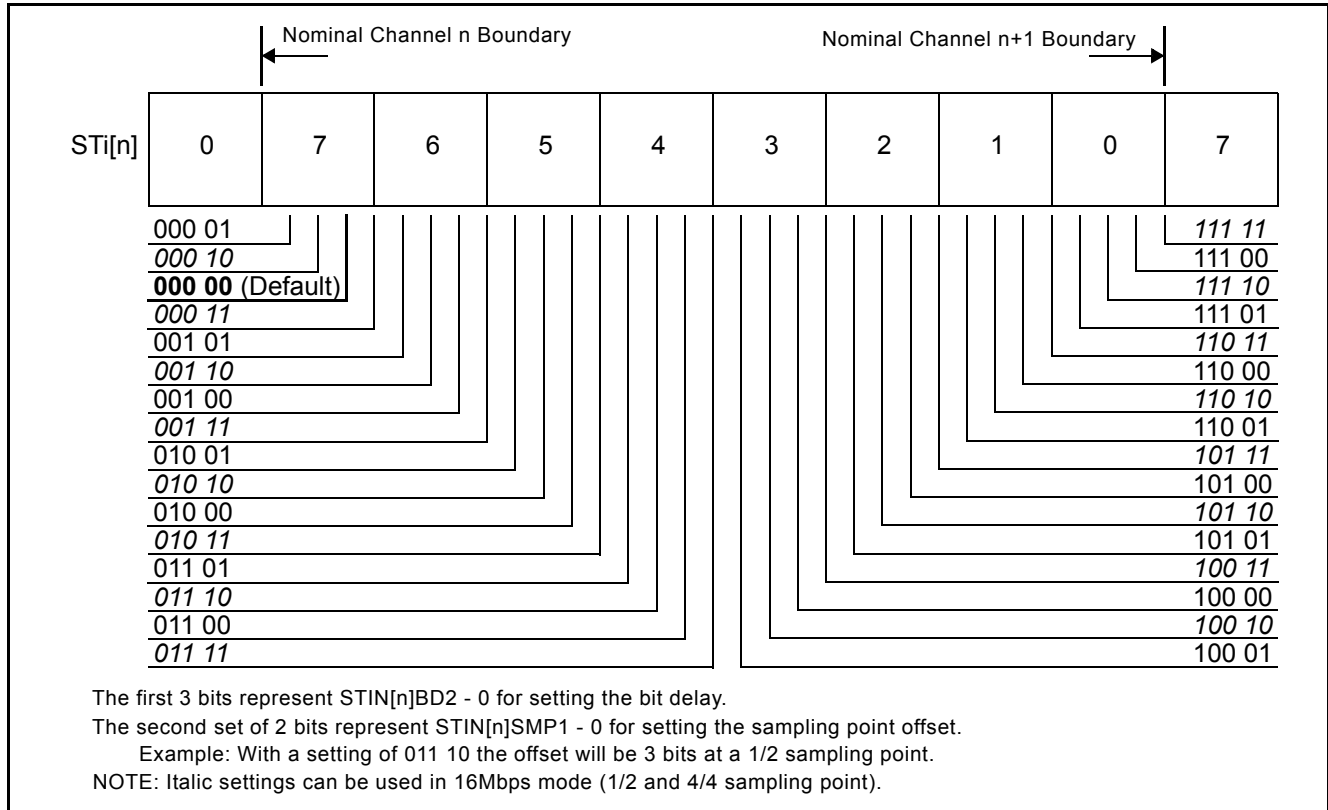
Figure 15 - Input Bit Delay and Factional Sampling Point
