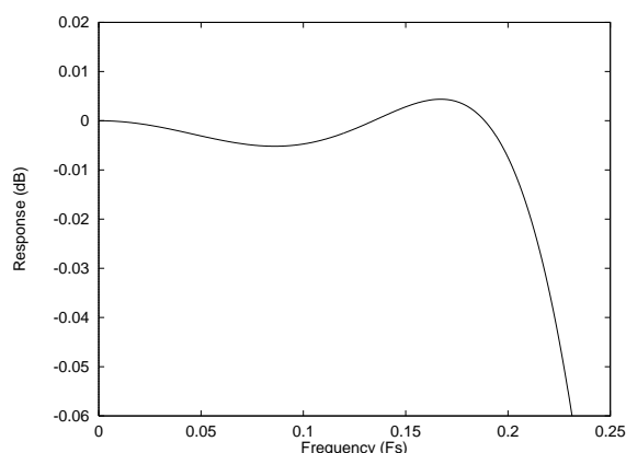
Figure 32 ADC Digital Filter Ripple –Type 2
