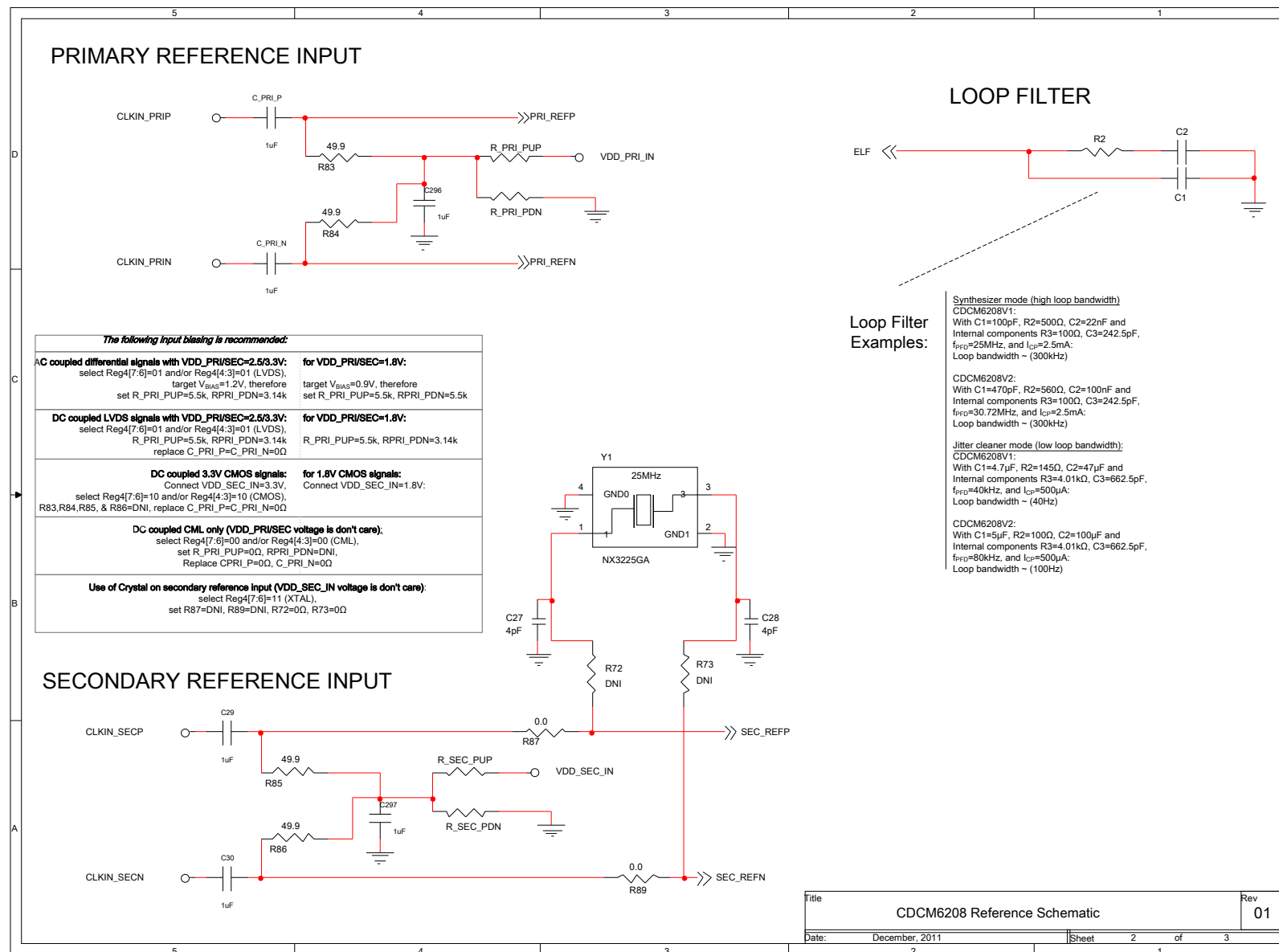
Figure 54. Schematic page 2
