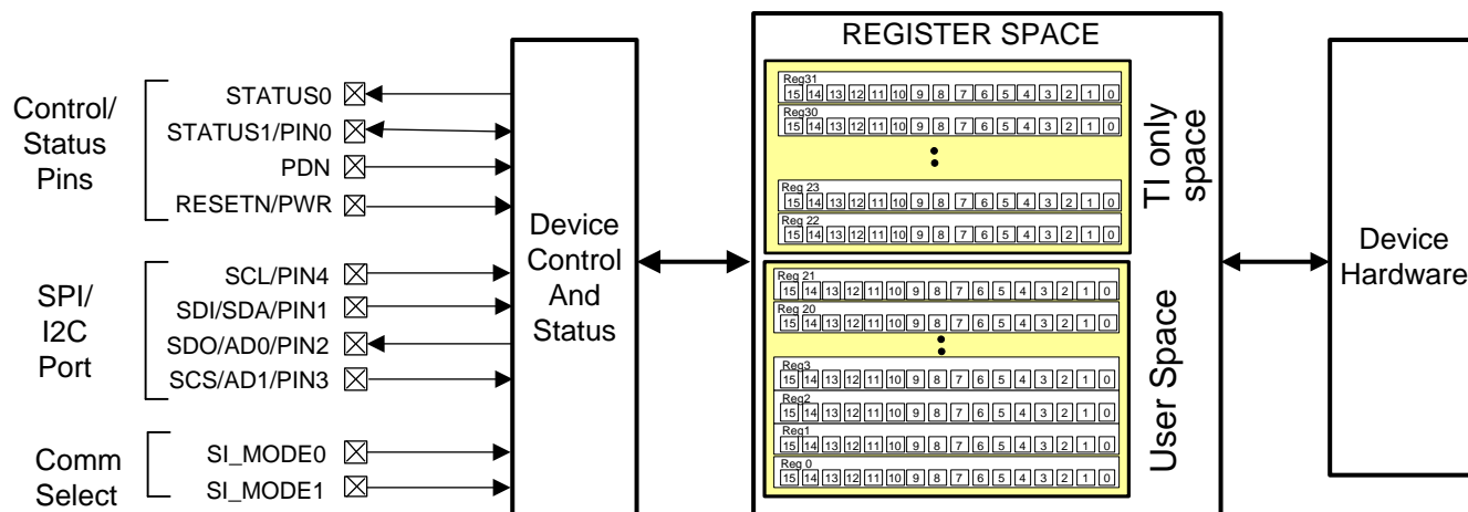
Figure 42. CDCM6208 Interface and Control Block
