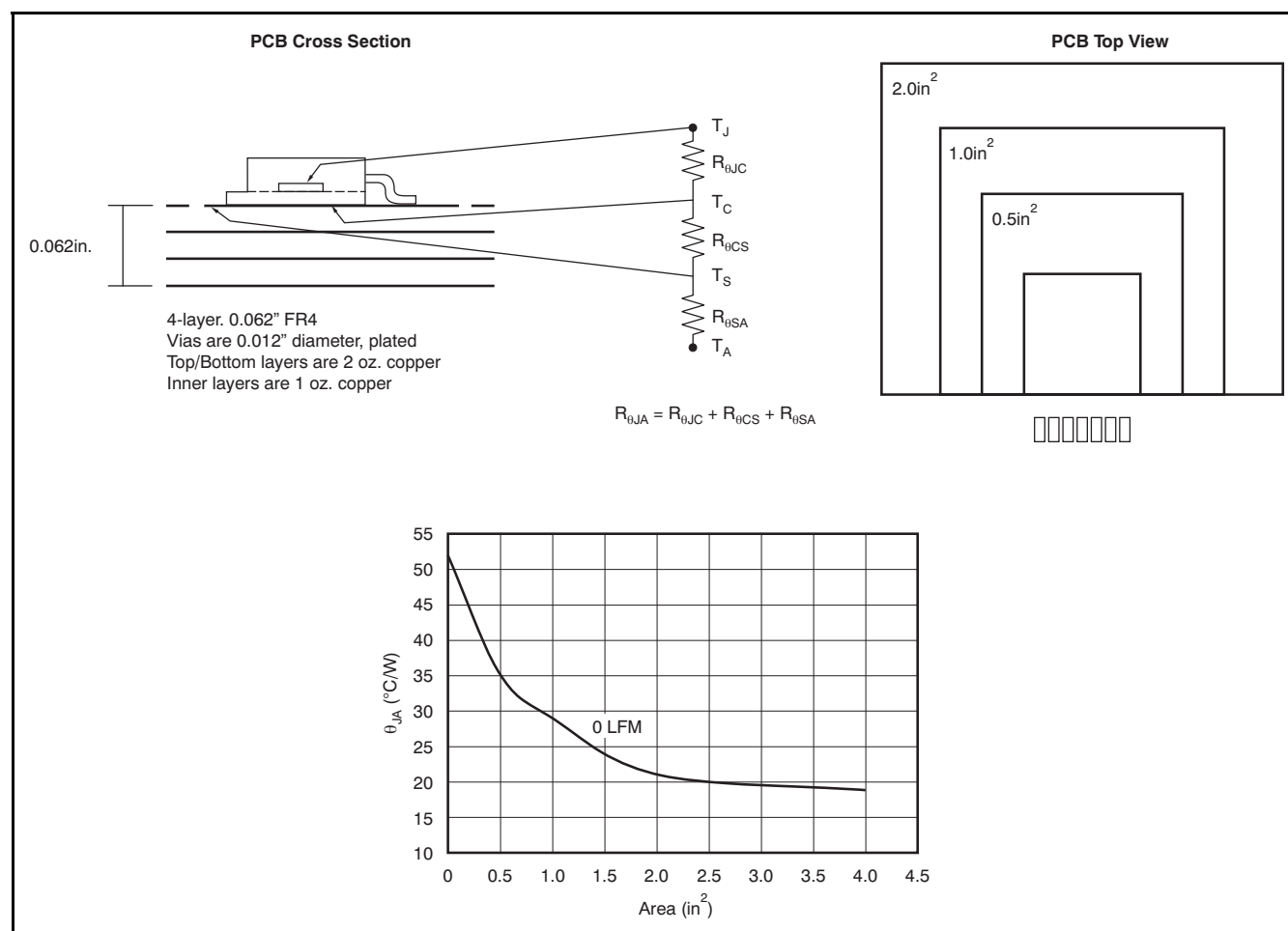
Figure 33. KTW (DDPAK-7) PCB Layout and Corresponding R_{\theta JA} , Top Layer Thermal Plane
