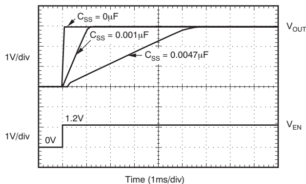
Figure 2. Turn-On Response
