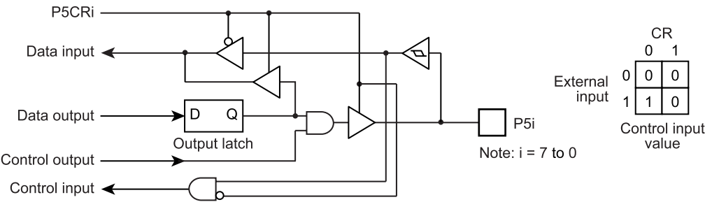
Figure 5-7 Port P5
