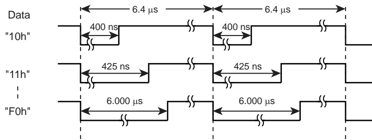
Figure 17-3 7-Bit Mode
