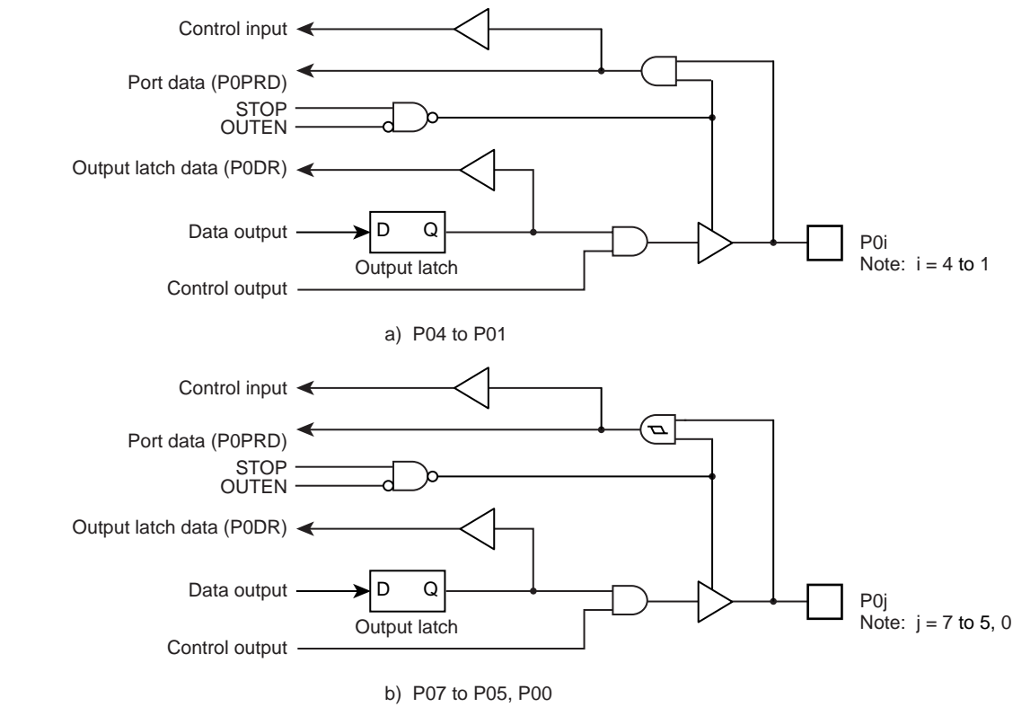
Figure 5-2 Port 0
