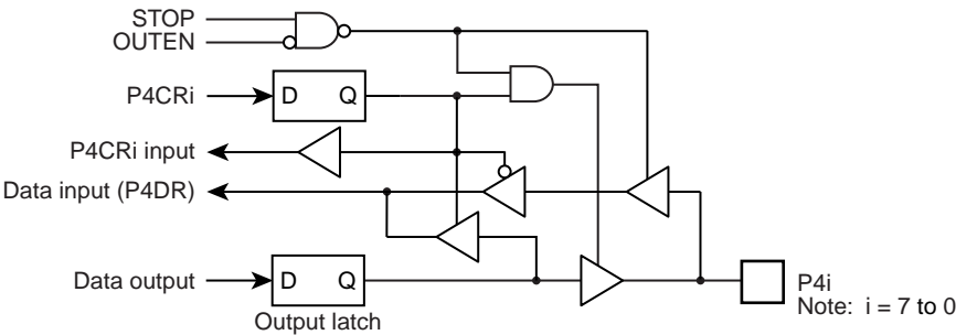
Figure 5-6 Port P4
