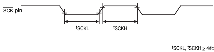
Figure 9-3 External Clock
