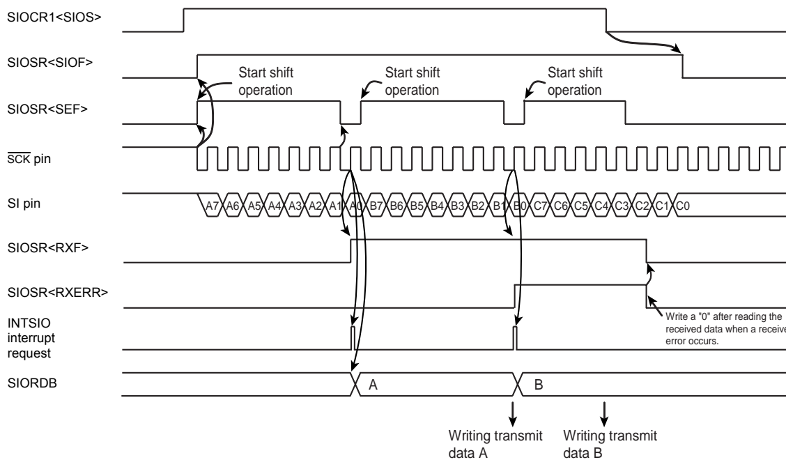
Figure 9-12 Example of Receive Error Processing
