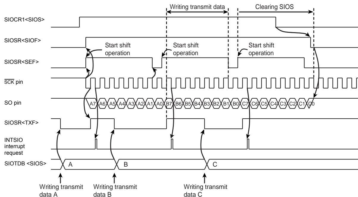
Figure 9-7 Example of External Clock and MSB Transmit Mode
