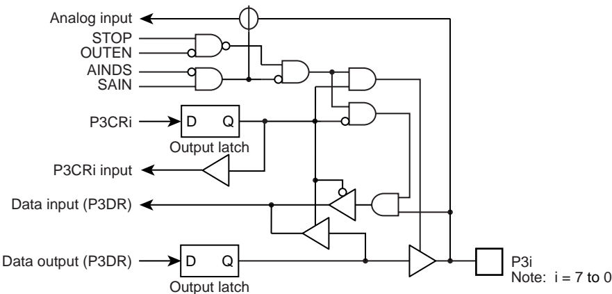
Figure 5-5 Port 3
