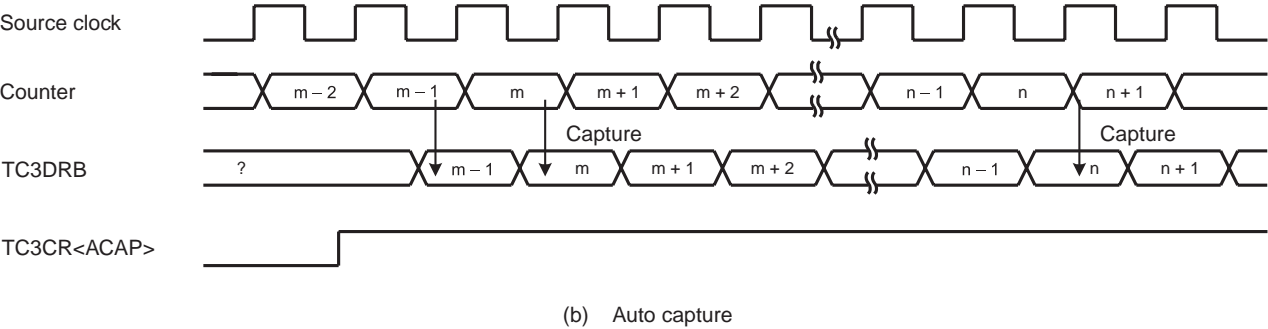
Figure 10-3 Timer Mode Timing Chart
