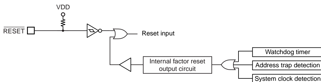
Figure 2-15 Reset Circuit
