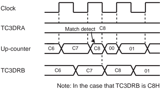
Figure 10-2 Auto-Capture Function
