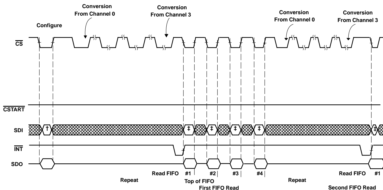
Figure 14. TLV2544/TLV2548 Mode 10/11 \mu\text{p} Serial Interface (Conversions Triggered by \overline{\text{CS}} )
