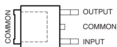
TL750L ... KVU PACKAGE (TOP VIEW)
