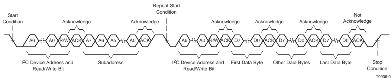
Figure 18. Multiple-Byte Read Transfer
