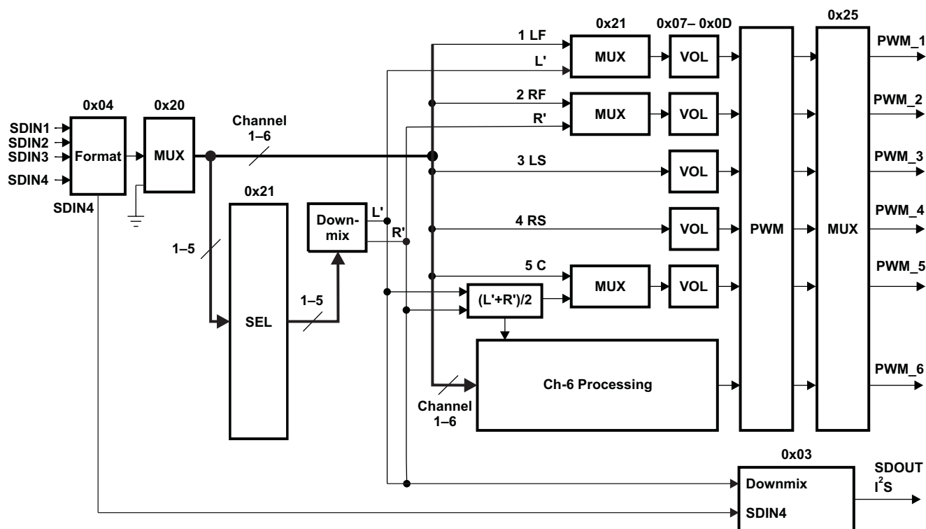
Figure 2. TAS5086 Data Flow Diagram With I 2 C Registers
