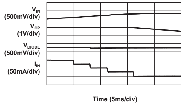
Charge Pump to Load Switch (2X Mode, 3x30mA Load)
