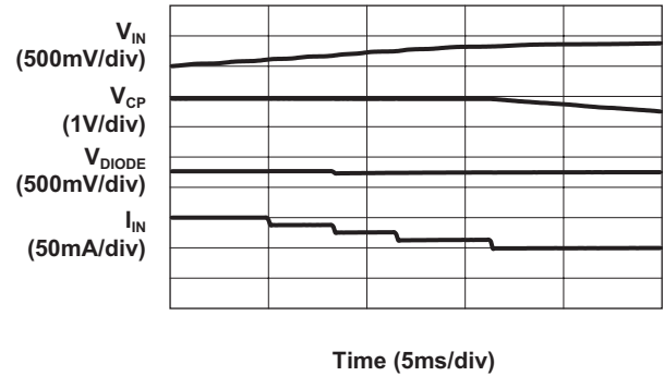
Charge Pump to Load Switch (1.5X Mode, 3x30mA Load)
