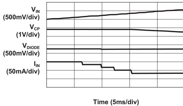
Charge Pump to Load Switch (2X Mode, 3x19mA Load)
