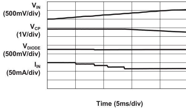
Charge Pump to Load Switch (1.5X Mode, 3x19mA Load)
