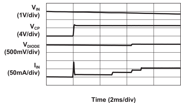
Load Switch to Charge Pump (1.5X Mode, 3x30mA Load)
