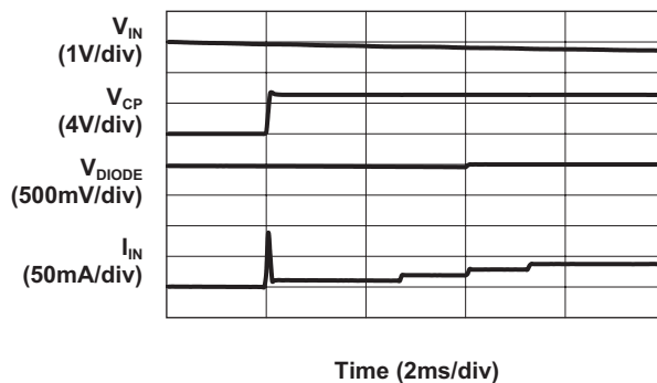
Load Switch to Charge Pump (1.5X Mode, 3x19mA Load)
