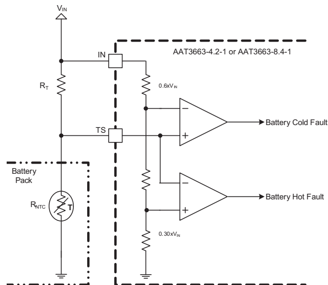
Figure 4: External Resistor and NTC Thermistor Application Circuit.
