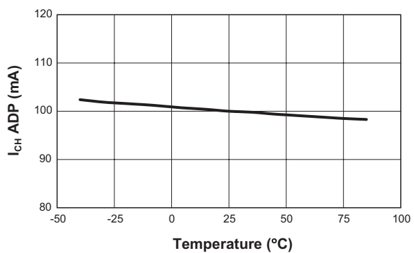
Preconditioning I_{CH} vs. Temperature (ADPSET = 8.06k \Omega )
