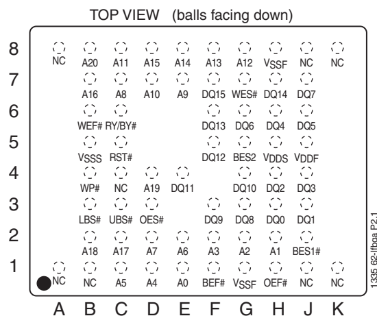
FIGURE 3: Pin Assignments for 62-ball LFBGA (8mm x 10mm)
