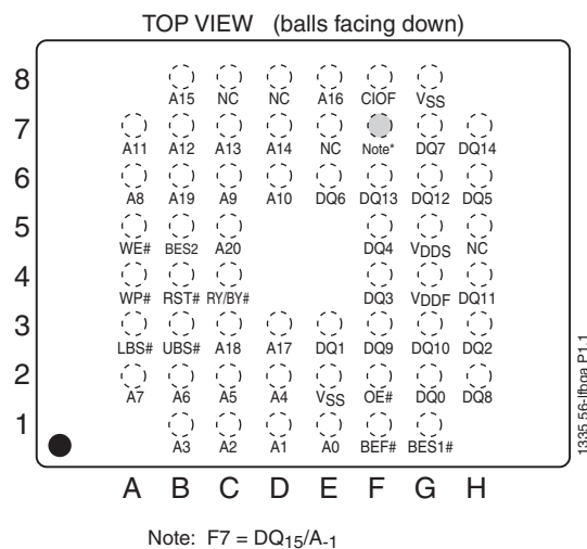
FIGURE 2: Pin Assignments for 56-ball LFBGA (8mm x 10mm)
