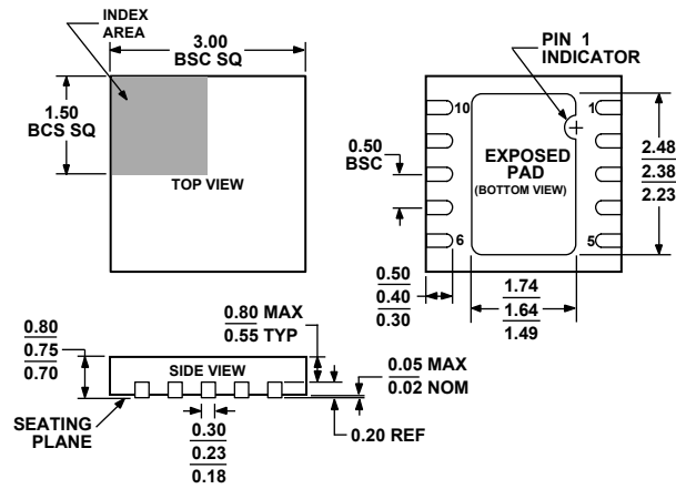
Figure 64. 10-Lead Lead Frame Chip Scale Package [LFCSP_WD] 3 mm x 3 mm Body, Very Very Thin, Dual Lead (CP-10-9) Dimensions shown in millimeters
