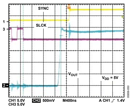
Figure 39. Exiting Power-Down to Midscale
