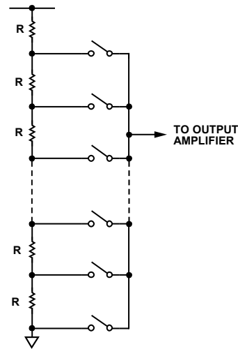
Figure 51. Resistor String
