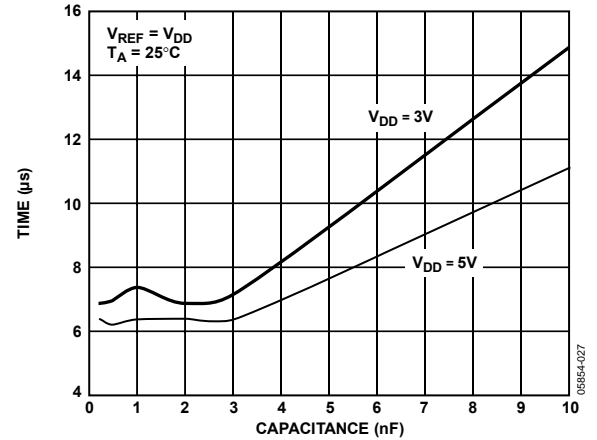
Figure 19. Settling Time vs. Capacitive Load
