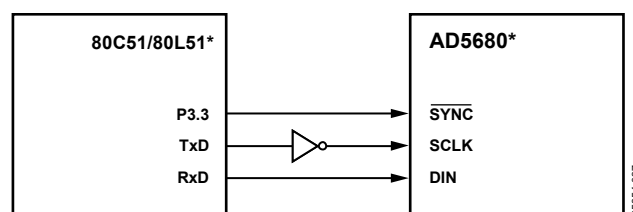
Figure 29. AD5680 to 80C51/80L51 Interface
