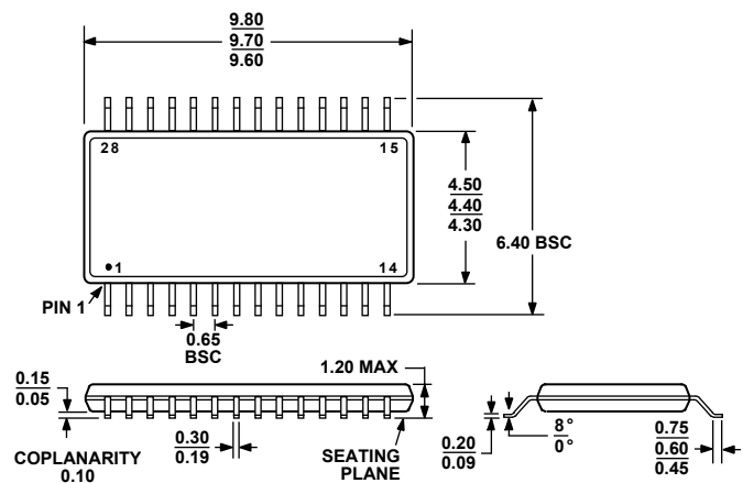
COMPLIANT TO JEDEC STANDARDS MO-153-AE Figure 49. 28-Lead Thin Shrink Small Outline [TSSOP] (RU-28) Dimensions shown in millimeters
