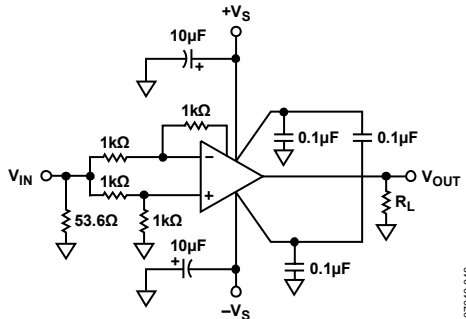
Figure 44. Common-Mode Rejection
