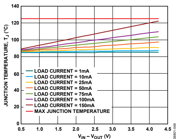
Figure 47. WLCSP, 100 mm² of PCB Copper, TA = 85°C
