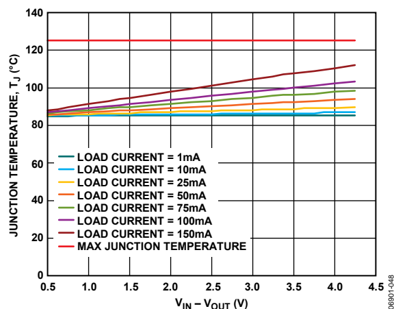
Figure 46. TSOT, 100 mm² of PCB Copper, TA = 85°C
