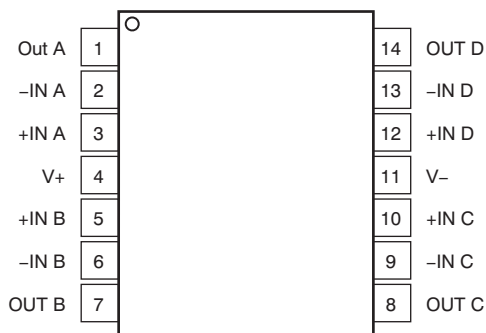
OPA4376 TSSOP-14 Top View
