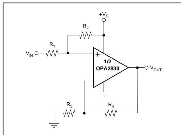
Figure 74. DC Level-Shifting
