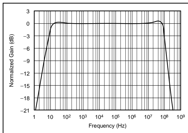
Figure 75. Video Line Driver Response to Matched Load
