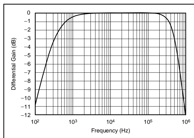
Figure 80. 5MHz, 2nd-Order, Butterworth Low-Pass Filter
