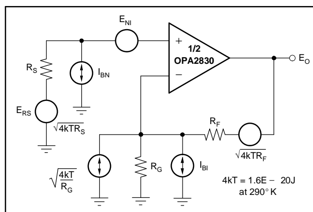
Figure 85. Noise Analysis Model
