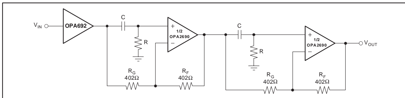
Figure 7. 2-Stage, All-Pass Network
