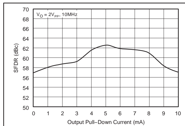
Figure 3. SFDR versus I_B
