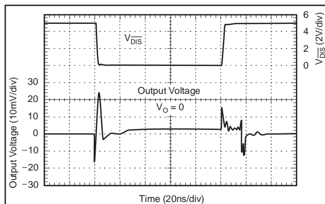
Figure 18. Disable/Enable Glitch
