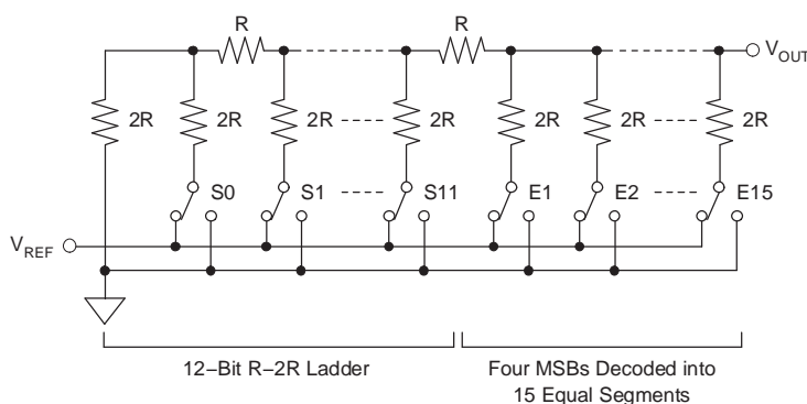
Figure 43. DAC Architecture
