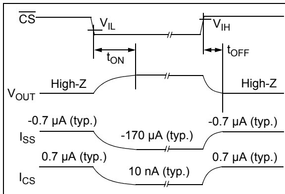
FIGURE 1-1: Timing Diagram for the Chip Select ( \overline{\text{CS}} ) pin on the MCP6273 and MCP6275.
