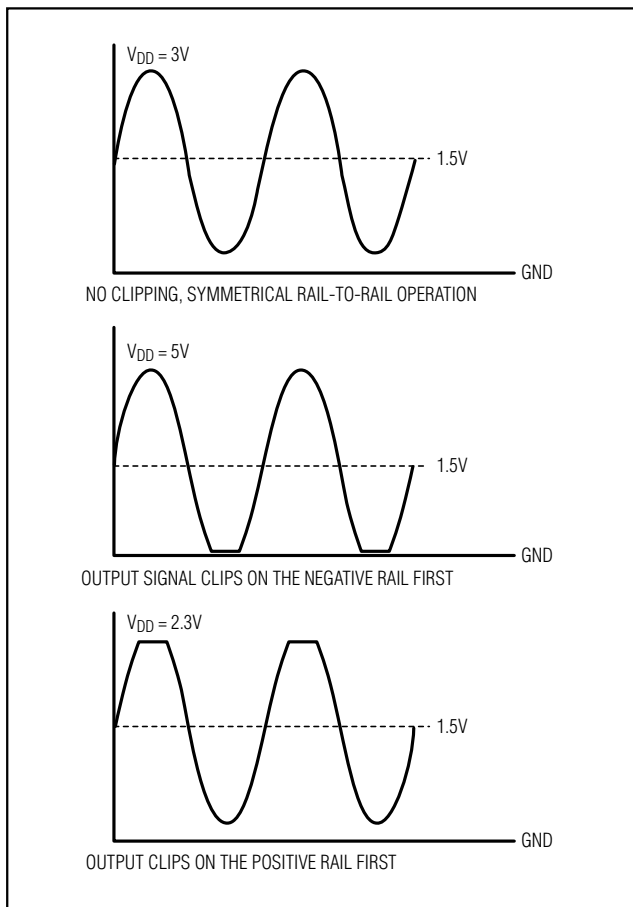
Figure 3. Rail-to-Rail Waveforms
