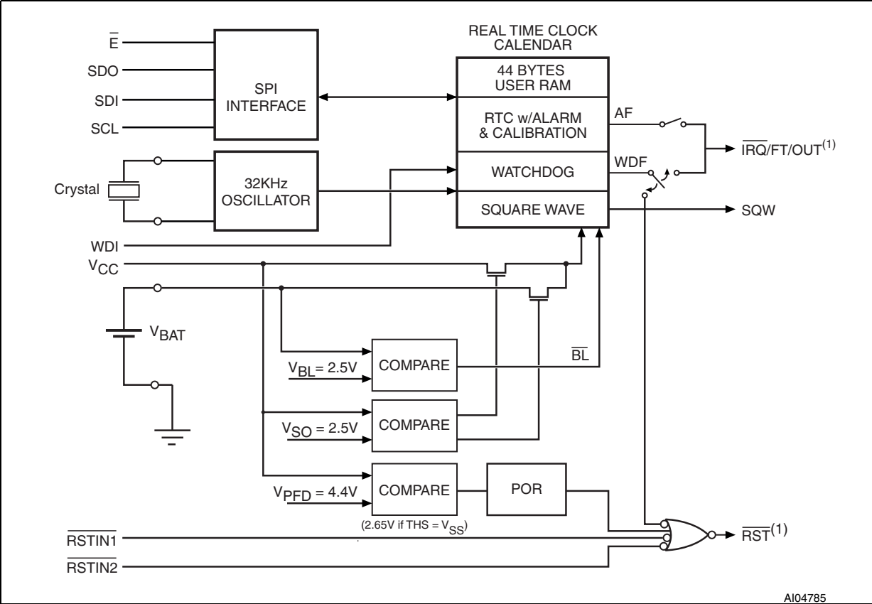
Figure 4. Block diagram
