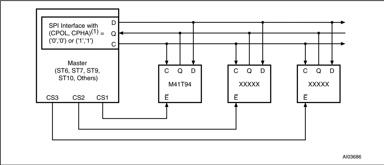
Figure 5. Hardware hookup
