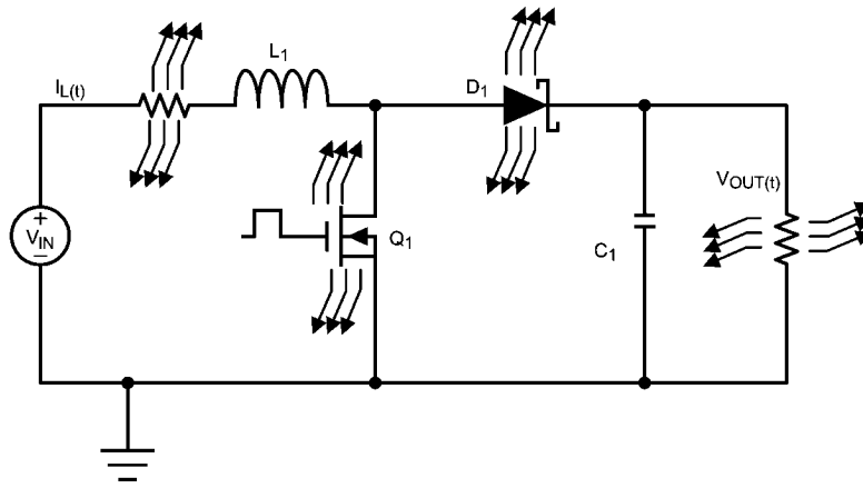
FIGURE 9. Thermal Schematic
