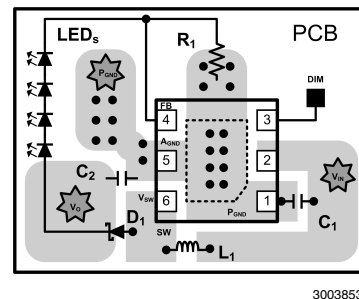
FIGURE 7. Boost PCB Layout Guidelines
