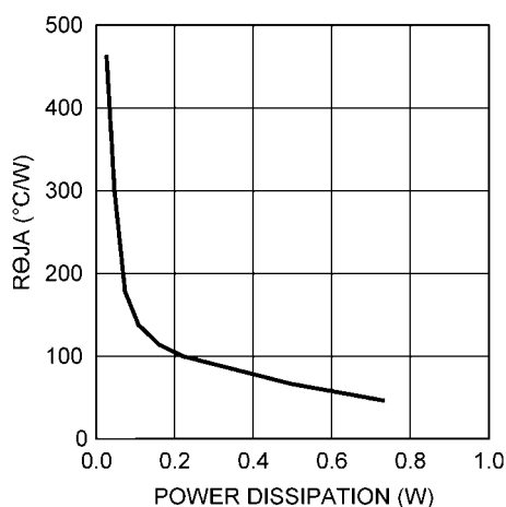
FIGURE 12. R θJA vs Internal Dissipation
