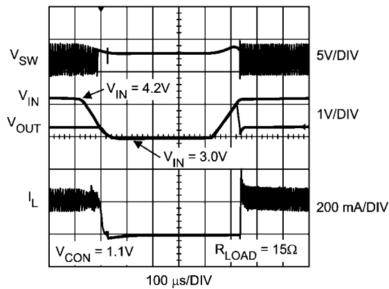
Automatic Bypass Operation ( V_{IN} = 4.2V to 3.0V )
