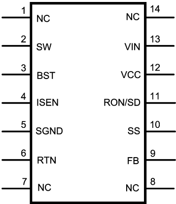
14-Lead TSSOP(EP)
