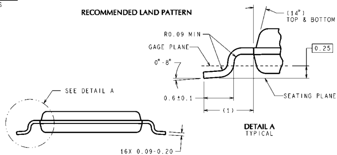
DIMENSIONS ARE IN MILLIMETERS 16-Lead ETSSOP Package NS Package Number MXA16A
