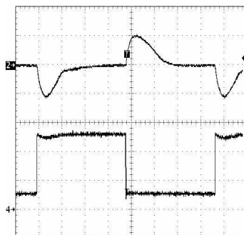
Figure 18. C_C = 4.7 nF
