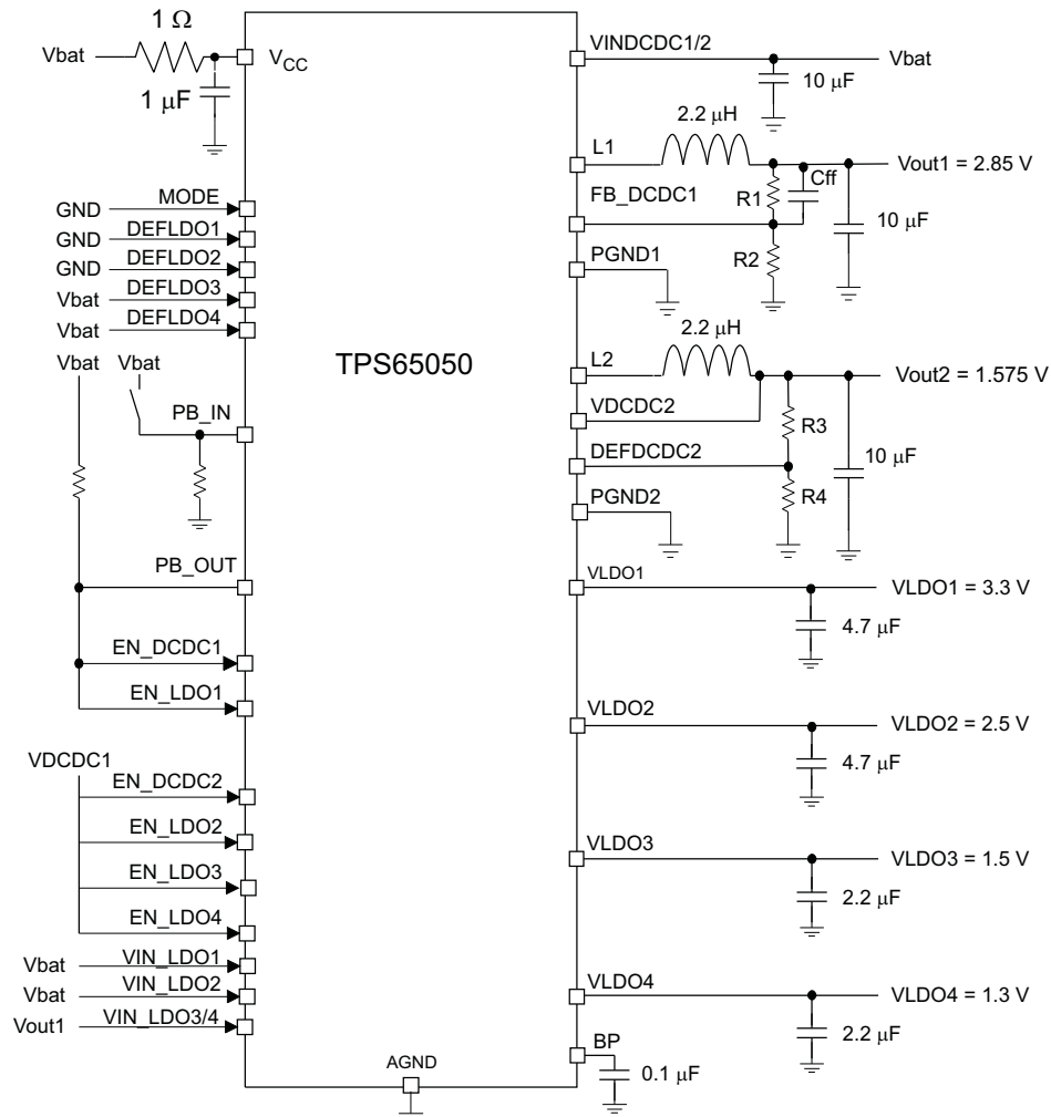
Figure 24. PB_ON/OFF Circuit
