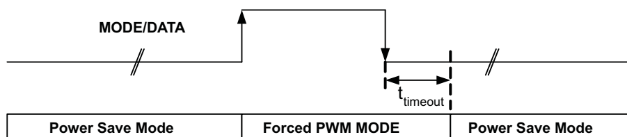
Figure 37. MODE/DATA PIN: Mode Selection
