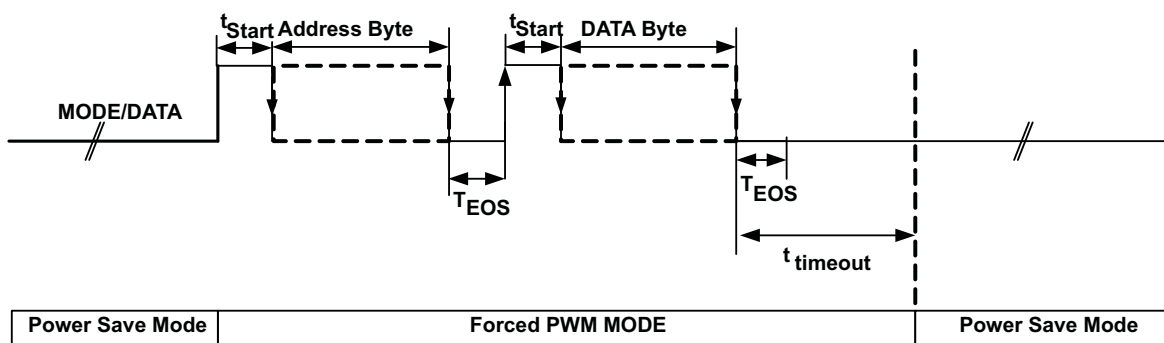
Figure 38. MODE/DATA Pin: Power Save Mode/Interface Communication
