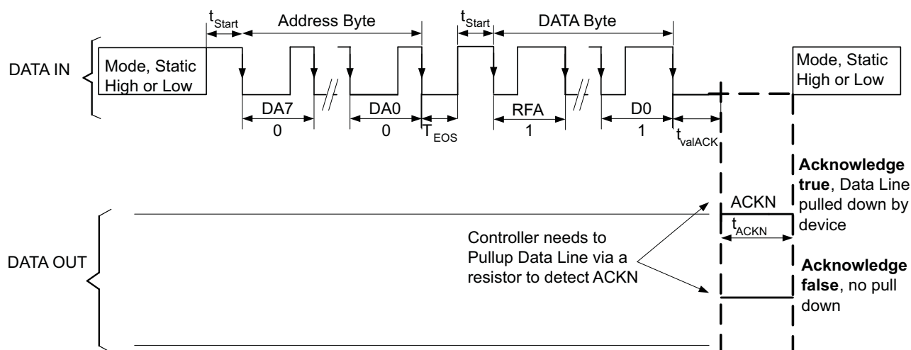
Figure 35. EasyScale™ Protocol Including Acknowledge
