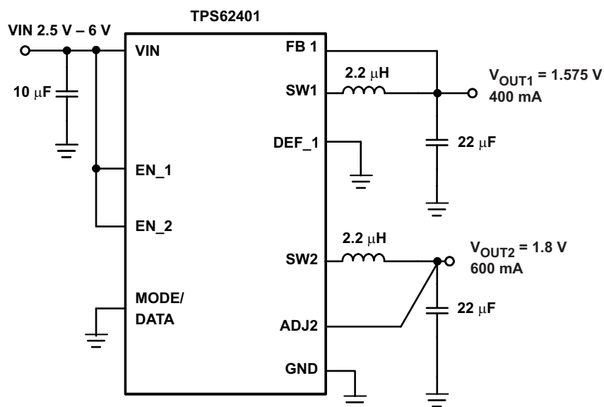
Figure 41. TPS62401 Fixed 1.575V/1.8V Outputs, low PFM Voltage Ripple Optimized
