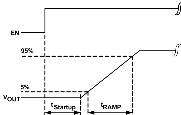
Figure 32. Soft Start
