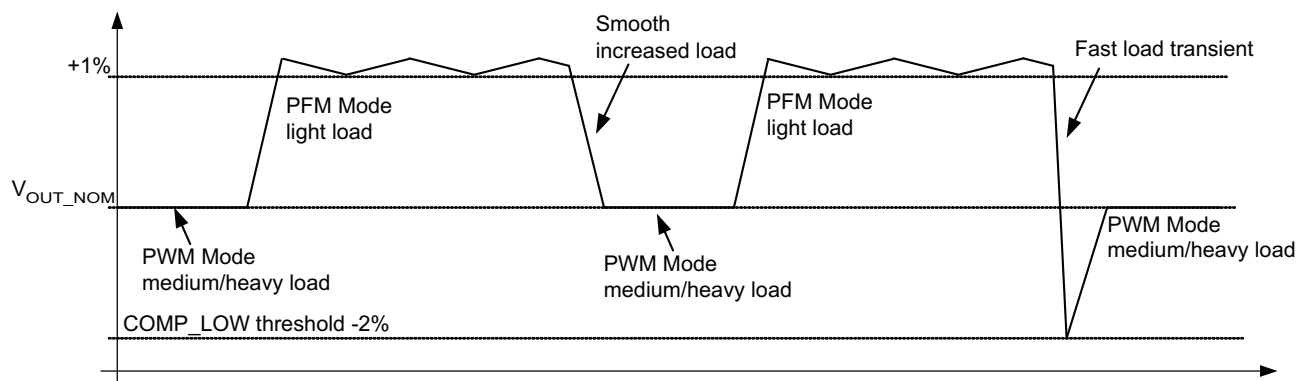
Figure 31. Dynamic Voltage Positioning
