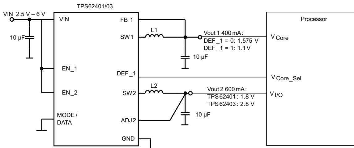
Figure 44. Dynamic Voltage Scaling on Vout1 Controlled by DEF_1 pin
