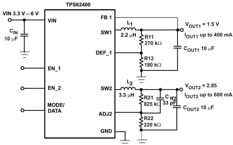
Figure 40. Typical Application Circuit 1.5V/2.85V Adjustable Outputs
