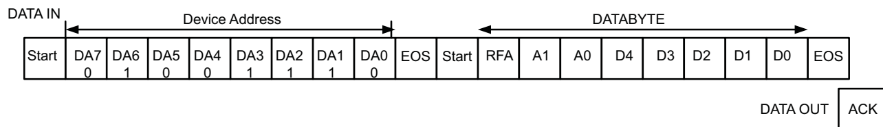
Figure 33. EasyScale™ Protocol Overview
