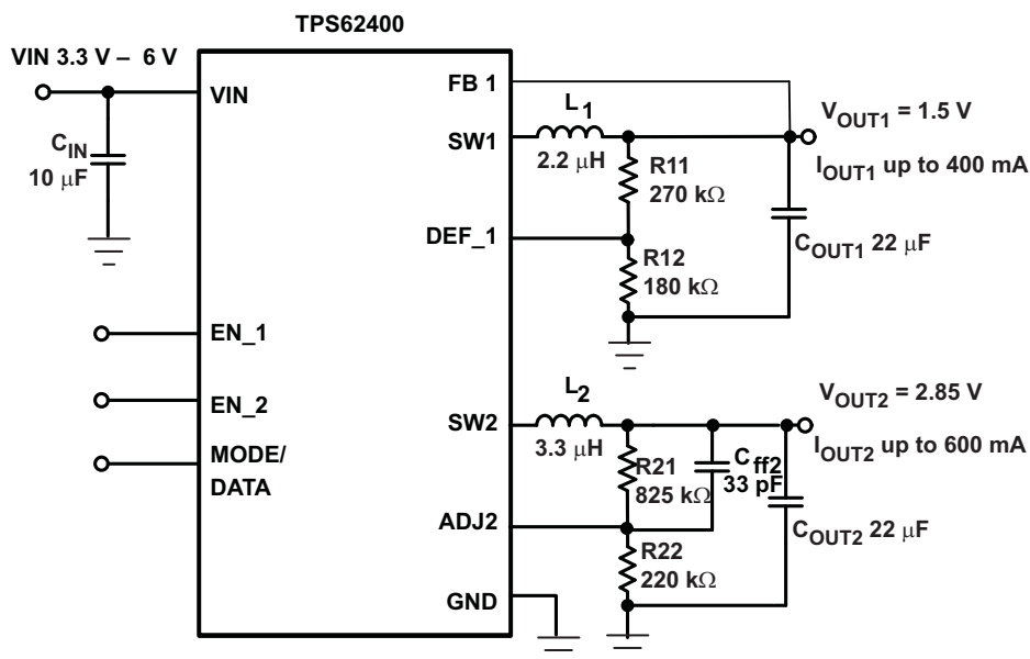
Figure 39. Typical Application Circuit 1.5V/2.85V Adjustable Outputs, low PFM Voltage Ripple Optimized
