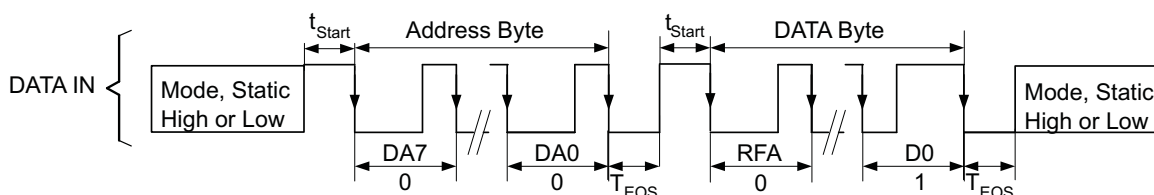
Figure 34. EasyScale™ Protocol Without Acknowledge
