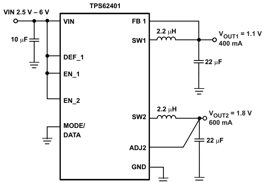
Figure 42. TPS62401 Fixed 1.1V/1.8V Outputs, low PFM Ripple Voltage Optimized
