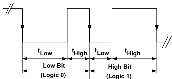
Figure 36. EasyScale™– Bit Coding
