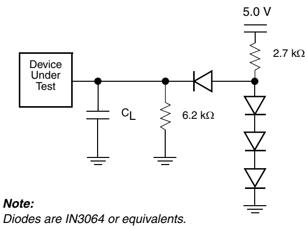
Figure 9. Test Setup
