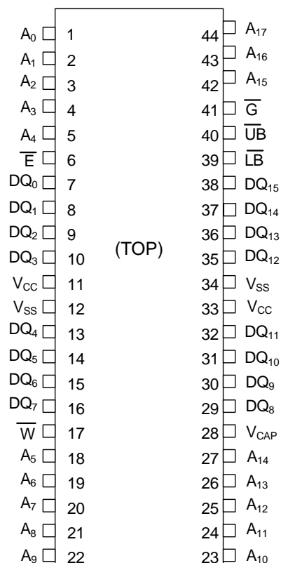
44-Pin TSOP-II
