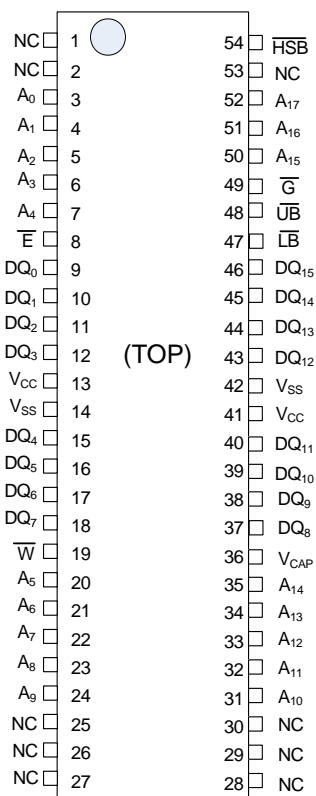
54-Pin TSOP-II
