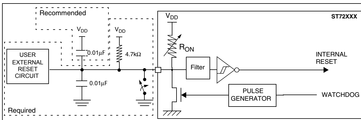
Figure 75. \overline{\text{RESET}} pin protection when LVD is disabled. 1)
