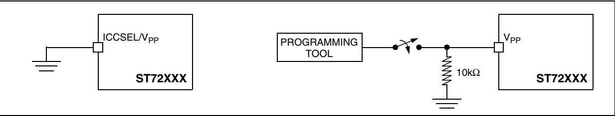
Figure 76. Two typical Applications with ICCSEL/V PP Pin 2)
