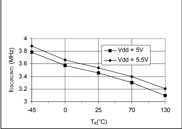
Figure 64. Typical f OSC(RCINT) vs T A
