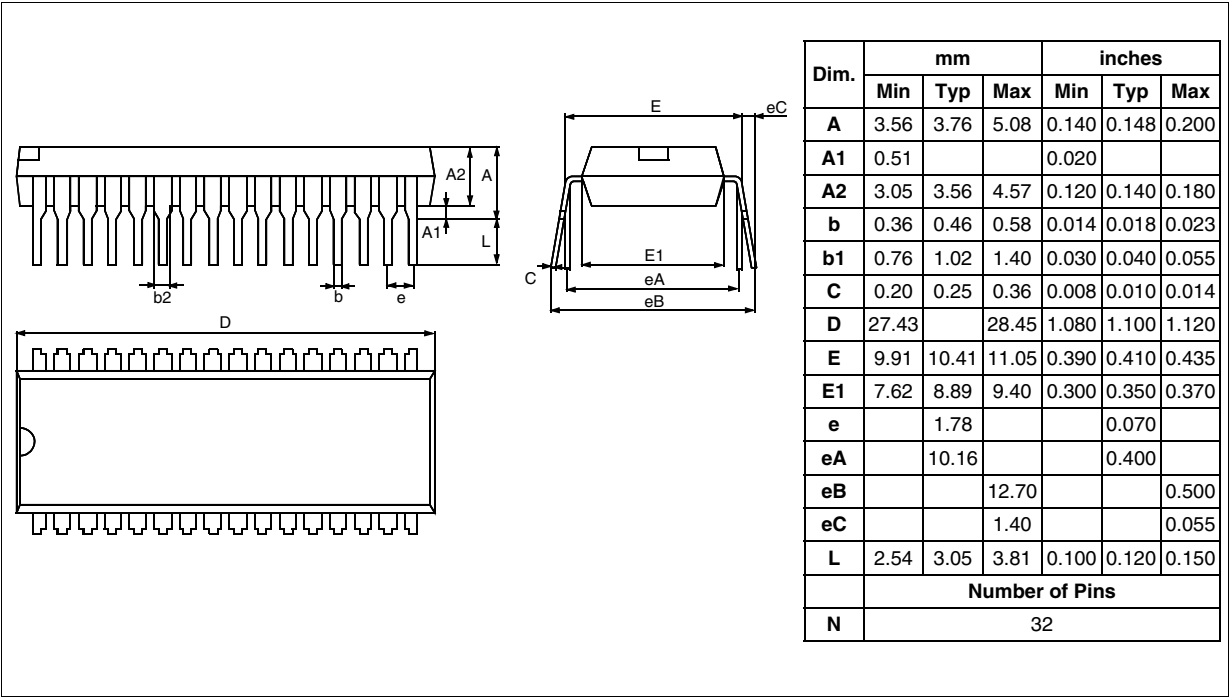
Figure 88. 32-Pin Plastic Dual In-Line Package, Shrink 400-mil Width
