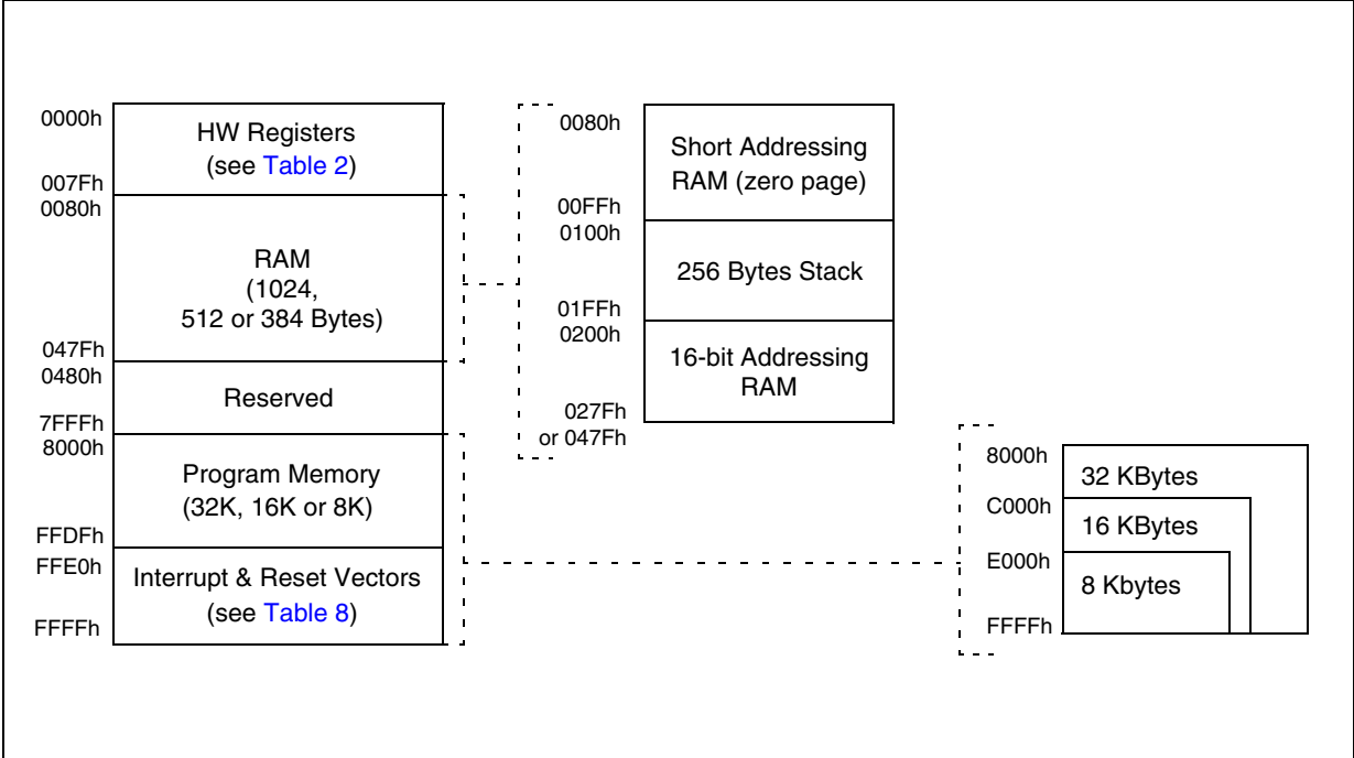
Figure 5. Memory Map
