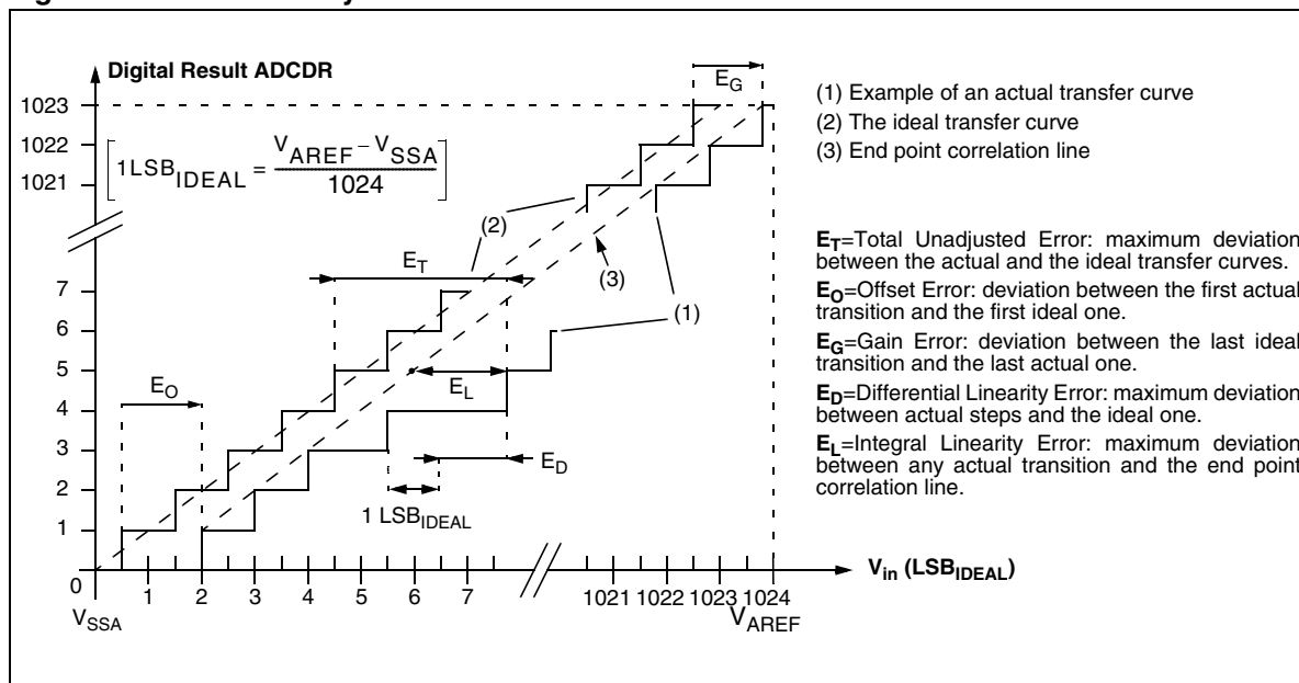
Figure 84. ADC Accuracy Characteristics
