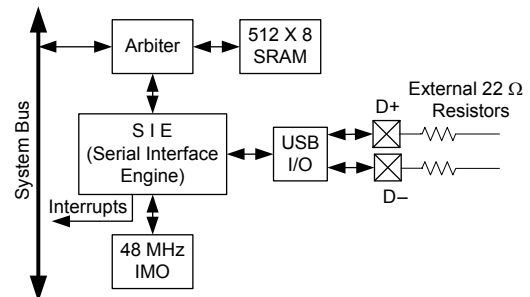
Figure 7-20. USB
