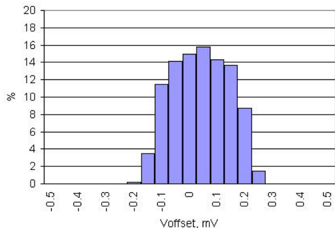
Figure 11-21. Opamp Voffset Histogram, 3388 samples/847 parts, 25 °C, Vdda = 5 V
