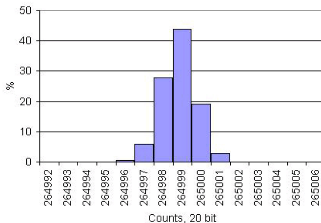
Figure 11-30. Delta-sigma ADC Noise Histogram, 1000 Samples, 20-Bit, 187 sps, Ext Ref, V_{IN} = V_{REF}/2 , Range = \pm 1.024 V
