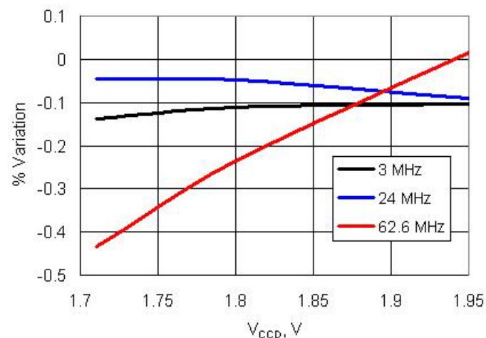
Figure 11-65. IMO Frequency Variation vs. V DD
