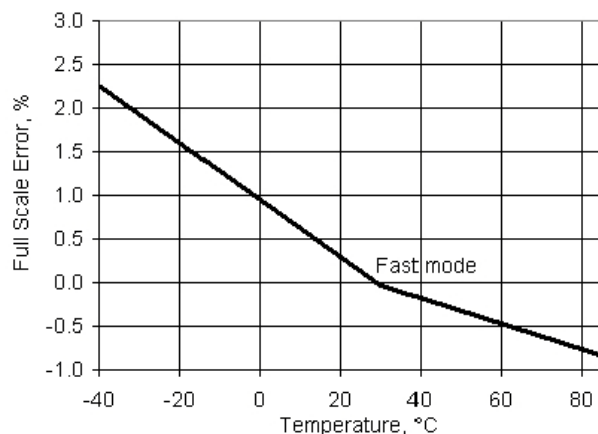
Figure 11-42. IDAC Full Scale Error vs Temperature, Range = 255 \mu A, Sink Mode
