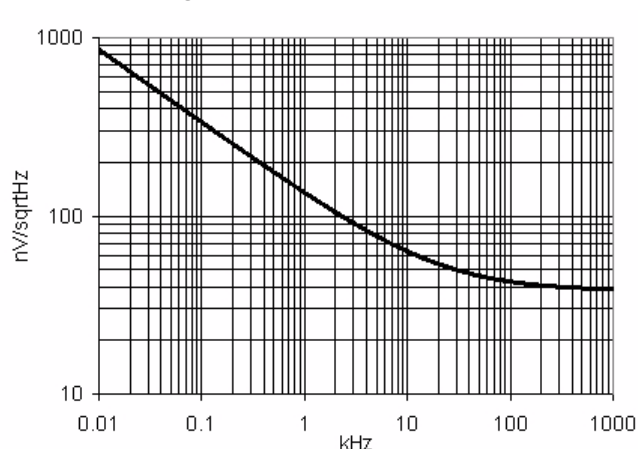
Figure 11-61. Noise vs. Frequency, V dda = 5 V, Power Mode = High
