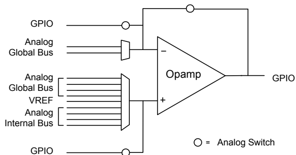
Figure 8-8. Opamp
