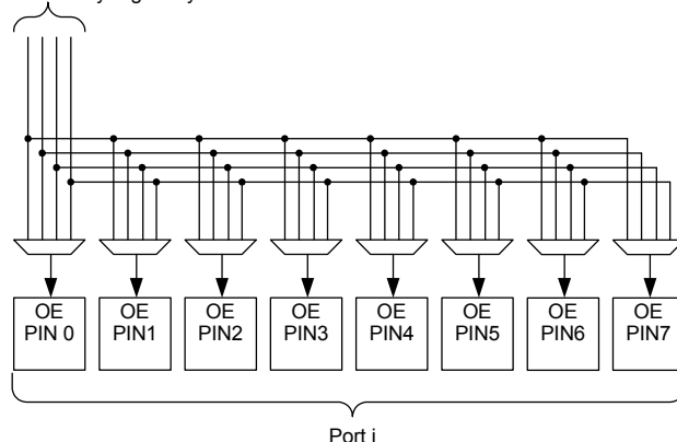
Figure 7-17. I/O Pin Output Enable Connectivity
