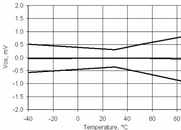
Figure 11-22. Opamp Voffset vs Temperature, Vdda = 5V
