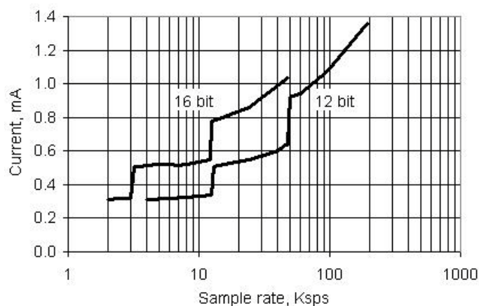
Figure 11-29. Delta-sigma ADC IDD vs sps, Range = \pm 1.024 V, Continuous Sample Mode, Input Buffer Bypassed
