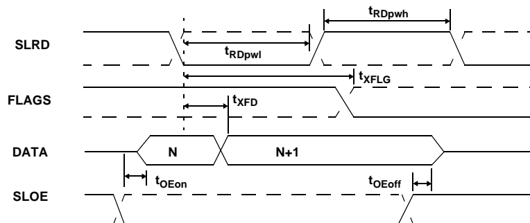
Figure 10. Slave FIFO Asynchronous Read Timing Diagram [17]
