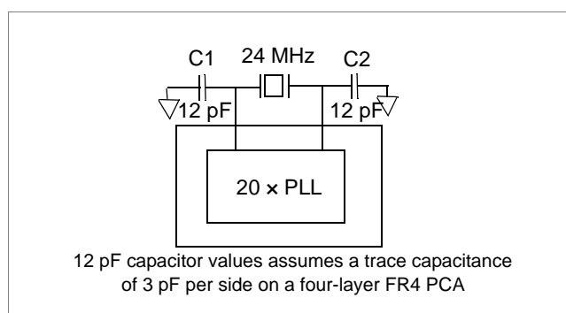
Figure 1. Crystal Configuration
