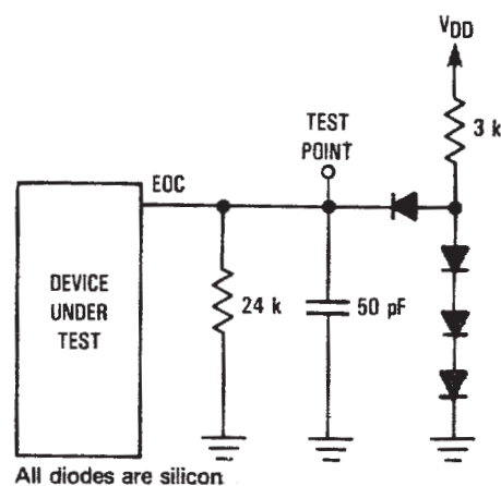
Figure 8. Test Circuit
