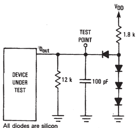
Figure 7. Test Circuit
