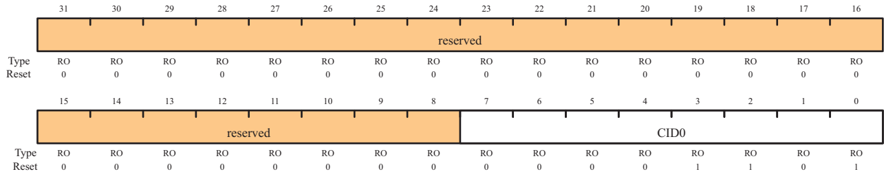
Watchdog Primecell Identification 0 (WDTPCellID0)
