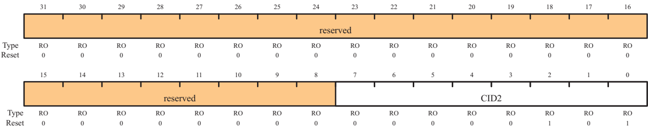
GPIO Primecell Identification 2 (GPIOCellIID2)
