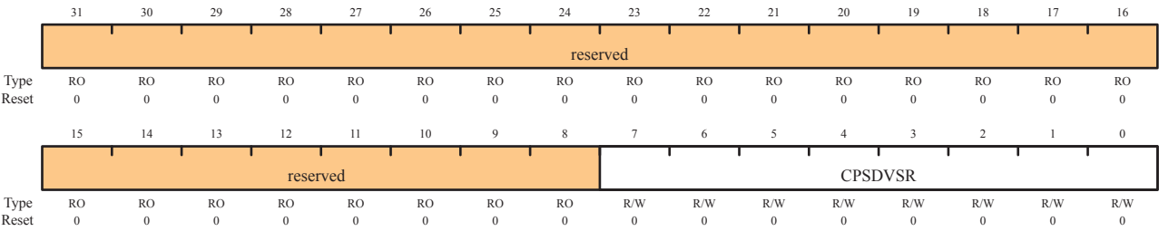
SSI Clock Prescale (SSICPSR)
