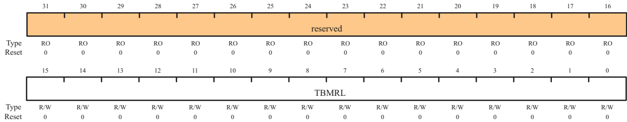
GPTM TimerB Match (GPTMTBMATCHR)
