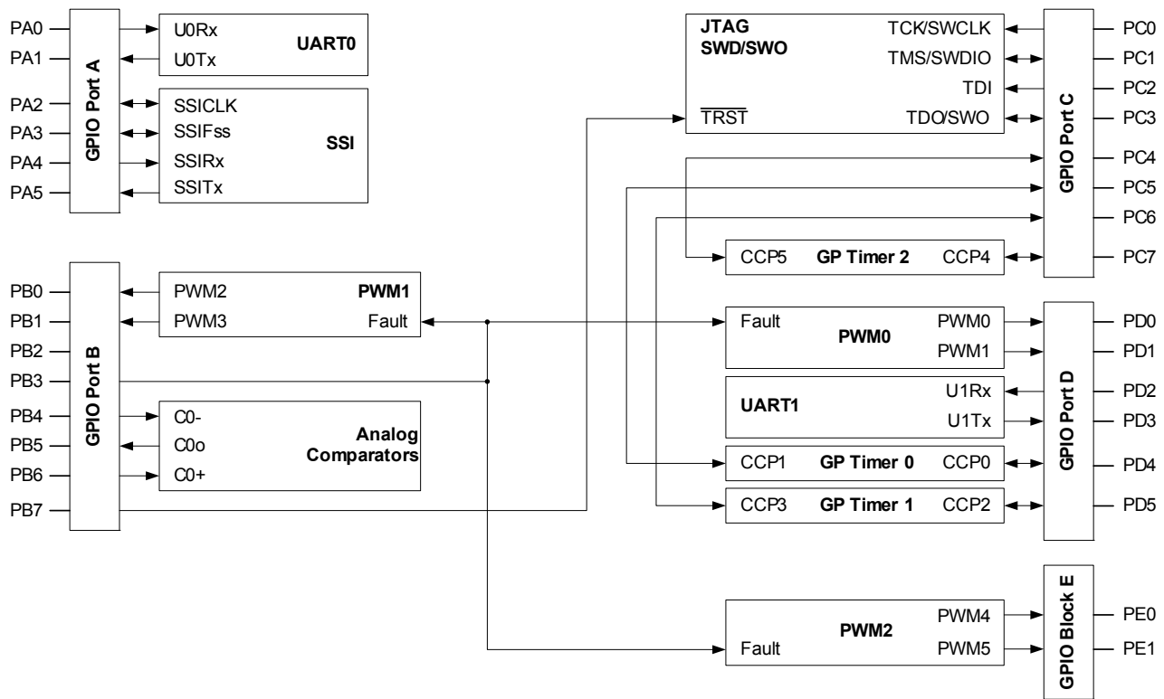
Figure 8-1. GPIO Module Block Diagram
