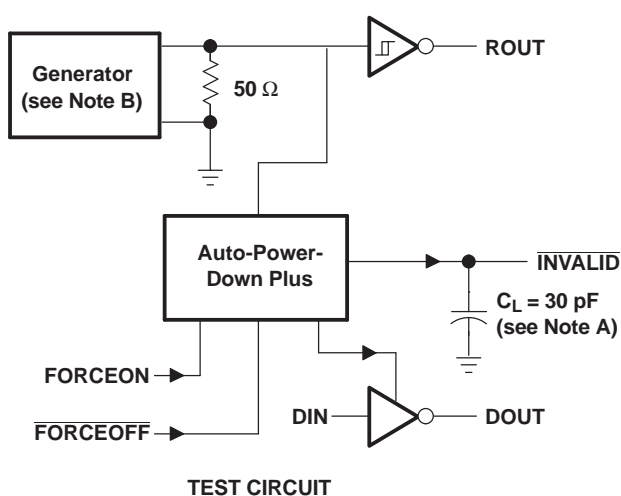
Figure 4. \overline{\text{INVALID}} Propagation Delay Times and Supply Enabling Time
